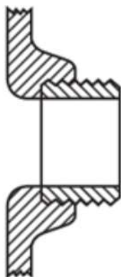
Outlet smooth and rounded (coef. 0.90)
