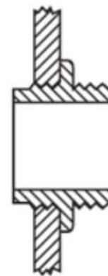
Outlet square and projecting into barrel (coef. 0.70)
