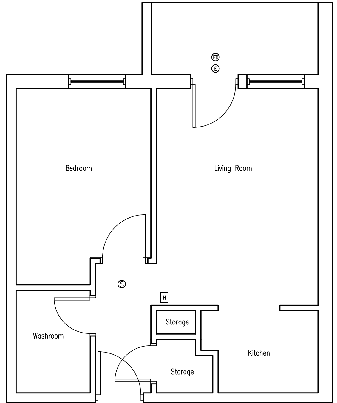
2 Second Floor Typical Suite 1/4" = 1'-0"
