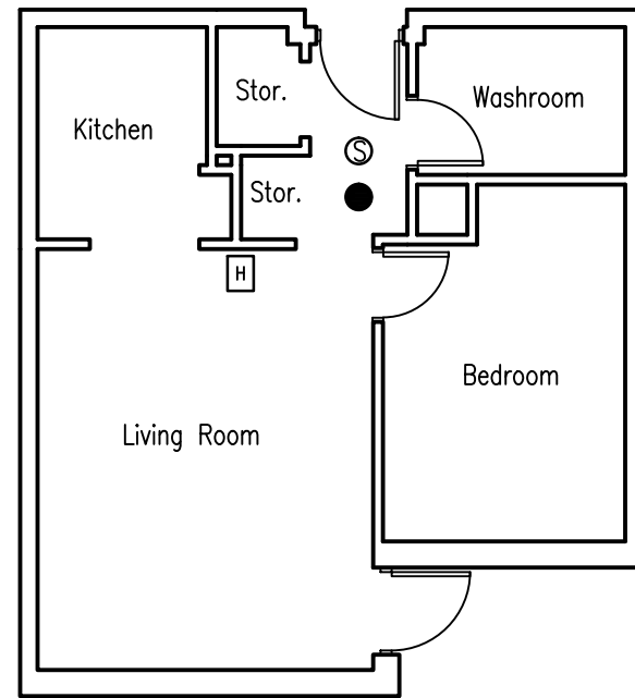
1 Typical Suite "A" 1/8" = 1'-0"
