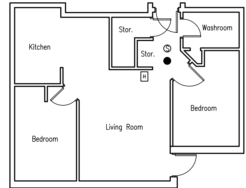
3 Typical Suite "Bx" 1/8" = 1'-0"
