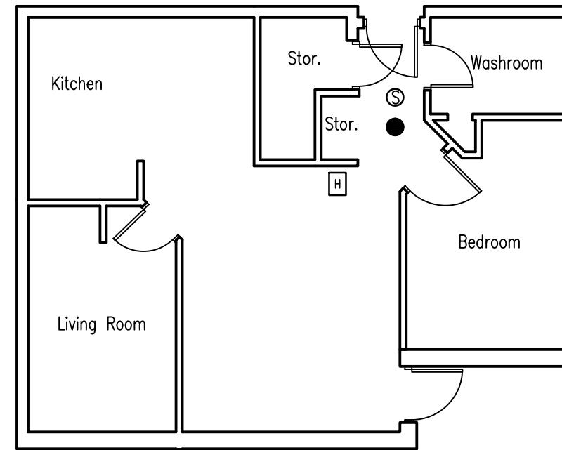
2 Typical Suite "B" 1/8" = 1'-0"
