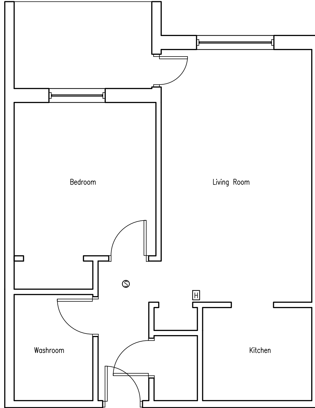
1 Typical Suite 1/4" = 1'-0"
