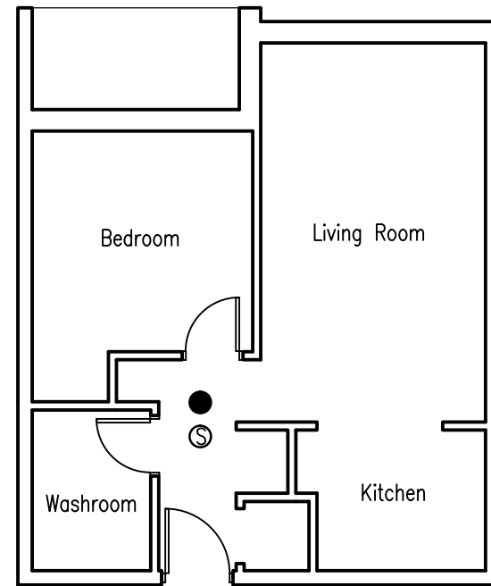
3 Typical Suite "B" 1/8" = 1'-0"
