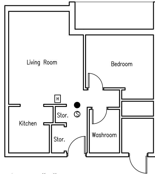
1 Typical Suite "A" 1/8" = 1'-0"
