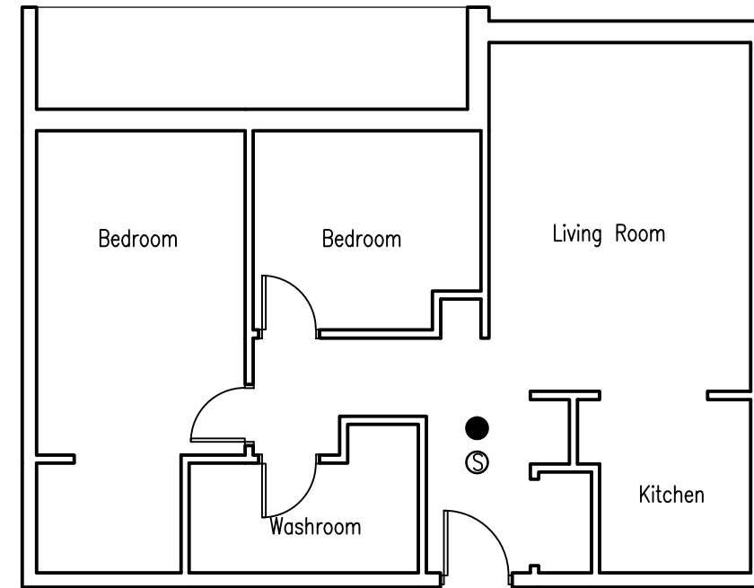
2 Typical B.F.A. Suite 1/8" = 1'-0"
