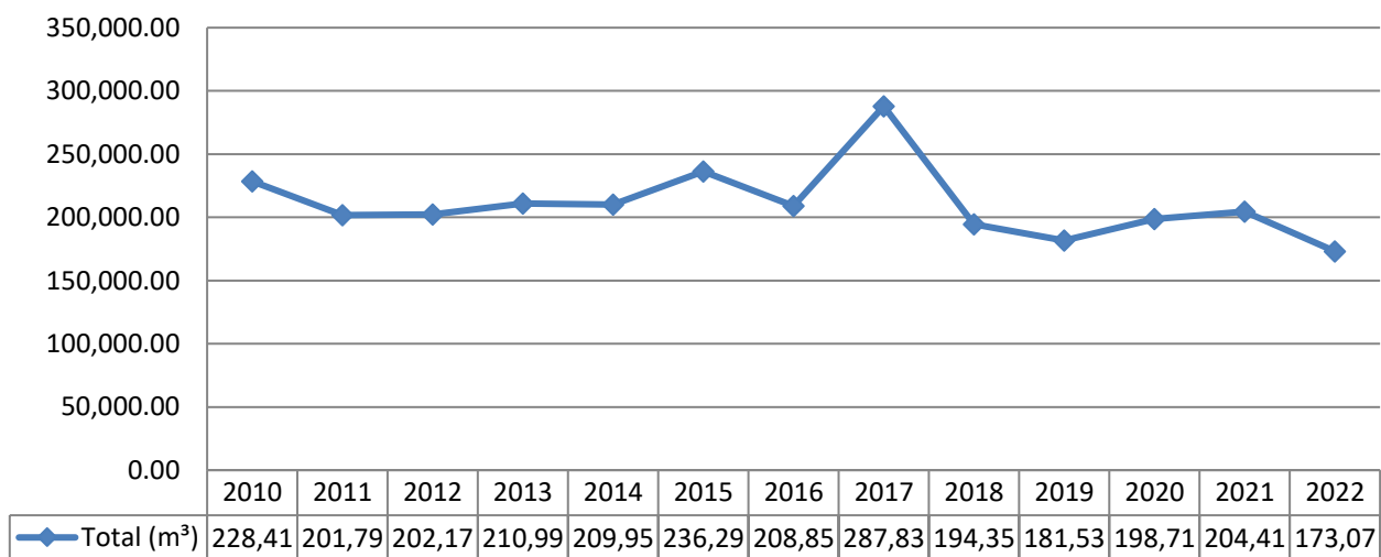
Graph 3: 2010 – 2022 Historical Influent Flows for the Omeme Sewage Lagoon
